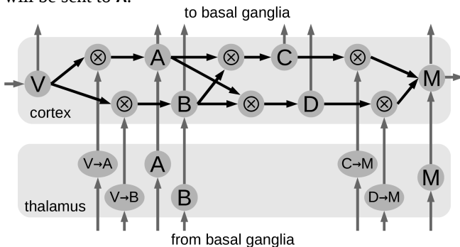
Figure 3: Thalamus and cortex model. Circles are 10,000 neurons representing 250 dimensional vectors ( V =vision; M =motor; A, B, C, D =working memory). \otimes are 40,000 neurons computing the binding operation.
