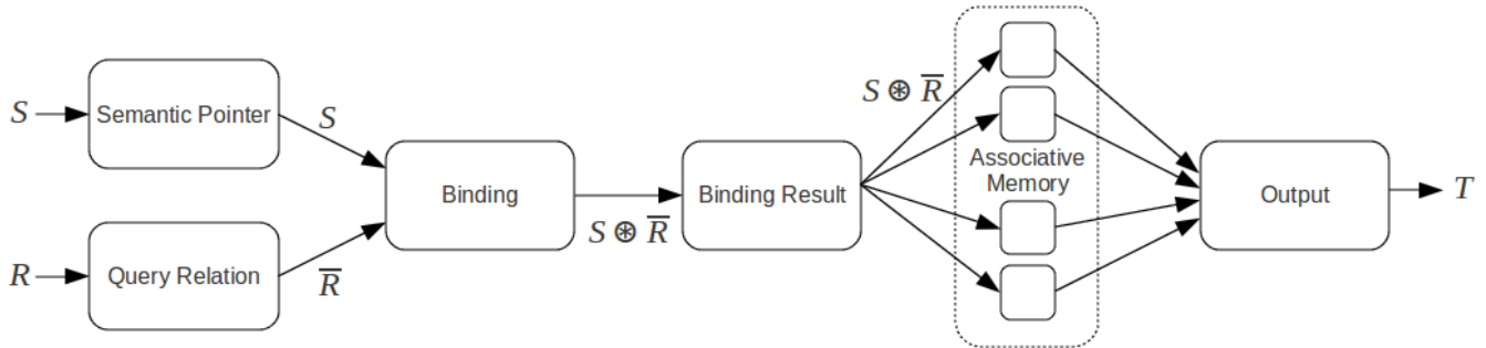
Figure 1: The network of spiking neurons that traverses the WordNet graph. Assume S = R \otimes T_{ID} + U \otimes V_{ID} where R , T_{ID} , U , and V_{ID} are all ID-vectors and T the semantic pointer corresponding to T_{ID} . All nodes correspond to populations of spiking neurons.
