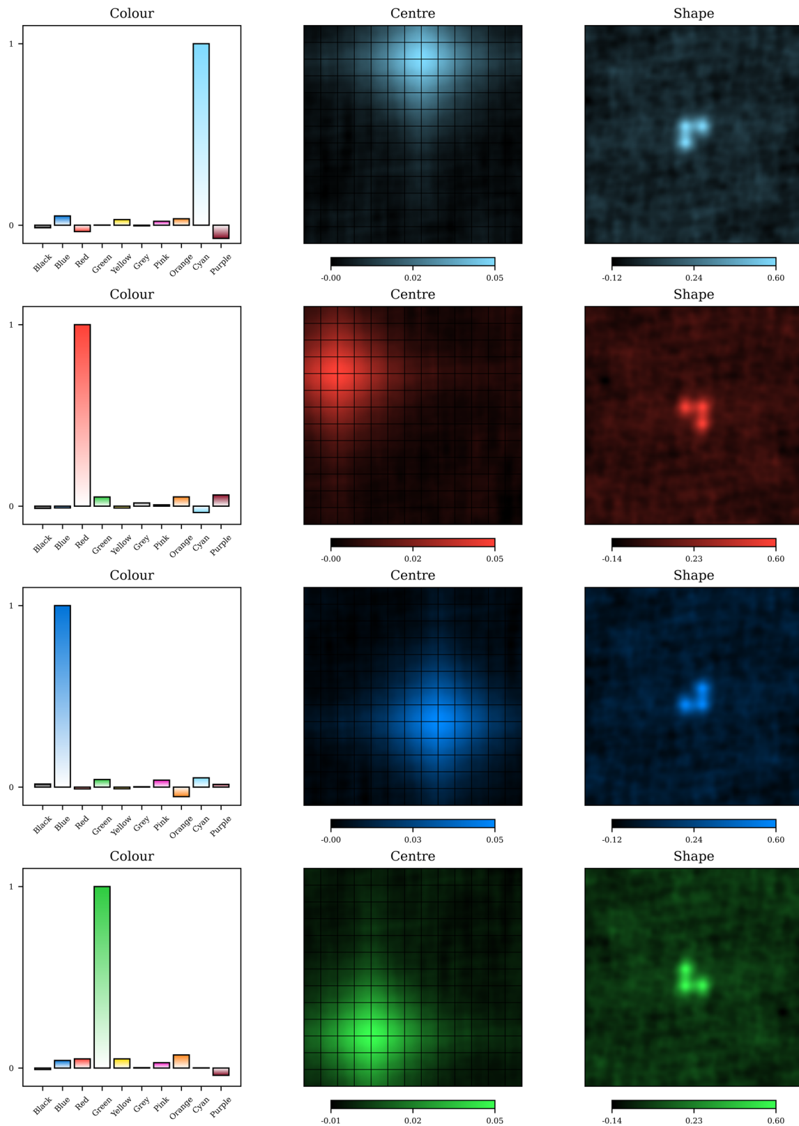
Fig. 5 | Visualization of the object representations for the input grid in the first demonstration of ARC-AGI task a61ba2ce (see Fig. 4). The colour subfigure (left) shows the similarity of the object's colour representation to each of the ten possible colour vectors. The centre subfigure (middle) shows the similarity of the
