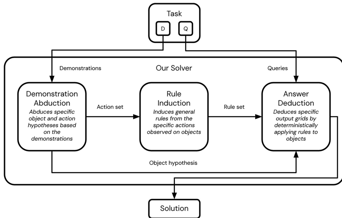
Fig. 7 | Our solver's general architecture.
