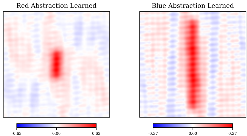
Fig. 9 | Visualization of the interpretation of the learned RECOLOUR parameter predictor NN for ARC-AGI task a61f2674 (see Fig. 3). The red subfigure (left) shows the prototype for objects recoloured red learned by the NN, determined here by the input object's shape property. The blue subfigure (right) shows the prototype for objects recoloured blue learned by the NN, again determined here by the input object's shape property. From these, we can verify the NN predicts red for short objects and blue for tall objects. These representations use N = 1024 -dimensional vectors.
