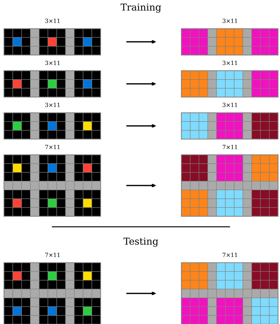
Fig. 2 | ARC-AGI task 54d9e175. Here, the implicit pattern is to colour each black region partitioned by the grey pixels according to the colour of the lone pixel at its centre (blue to pink, red to orange, green to cyan, and yellow to purple).
