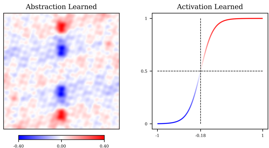
Fig. 8 | Visualization of the interpretation of the learned RECOLOUR operation predictor NN for ARC-AGI task a61f2674 (see Fig. 3). The abstraction subfigure (left) shows the prototype learned by the NN, determined here by the input object's shape property. The activation subfigure (right) shows the decision nonlinearity learned by the NN. From these, we can verify the NN selects for short and tall objects. Short objects' shape representations exist only in the centre, producing near-zero similarity mapping onto a likely probability. Medium-height objects' shape representations reach the negative similarity regions indicated by blue, producing a negative similarity mapping onto an unlikely probability. Finally, tall objects' shape representations reach the positive similarity regions indicated by red, producing a net positive similarity mapping onto a likely probability. These representations use N = 1024 -dimensional vectors.
